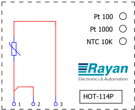
Wall/Outdoor Temperature Sensor
