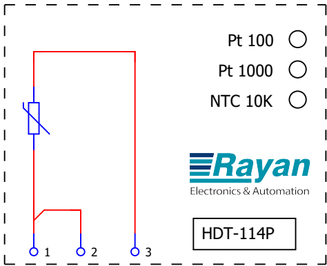
Duct Temperature Sensor
